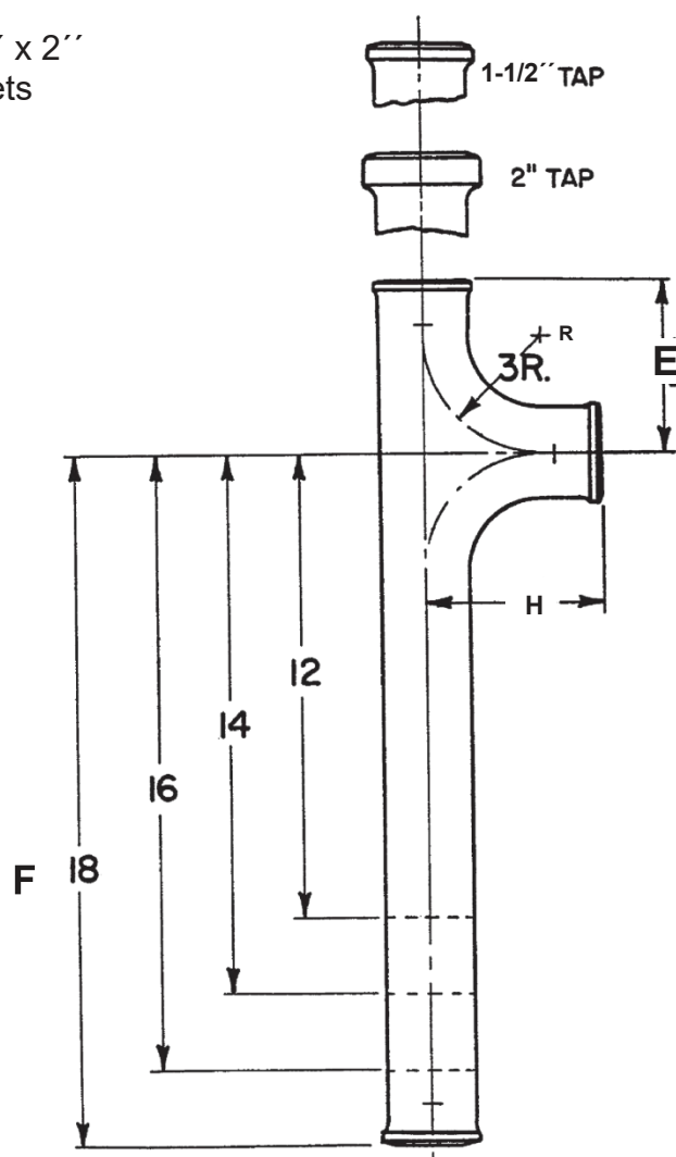
DOUBLE SWEEP SANITARY TEE (EXTENDED)
