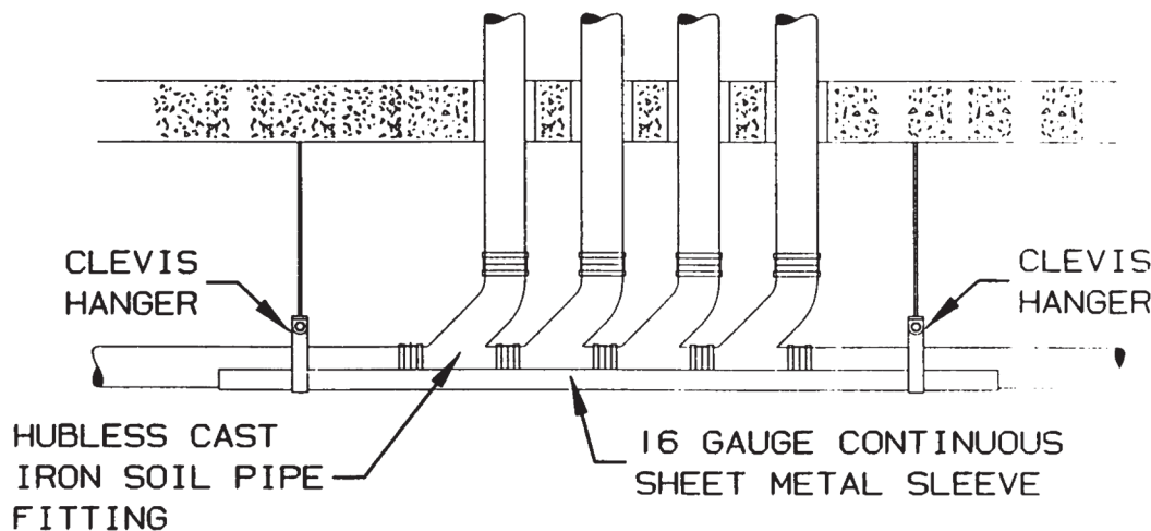
METHOD OF SUPPORTING "MULTI-FITTING" INSTALLATIONS (HANGER SPACING 10 ft. MAX.)
